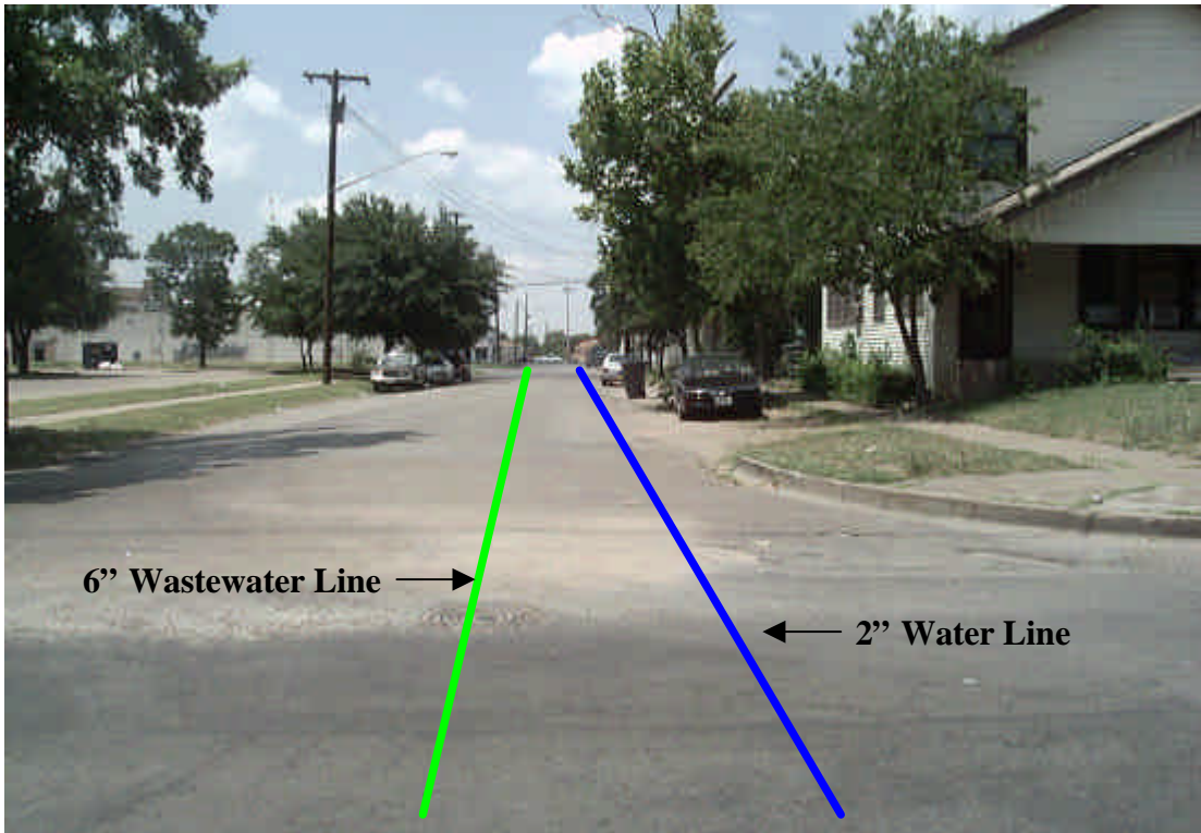
Figure 1 – Looking northwest at the wastewater manhole in Twelfth Street down Cumberland Street.
