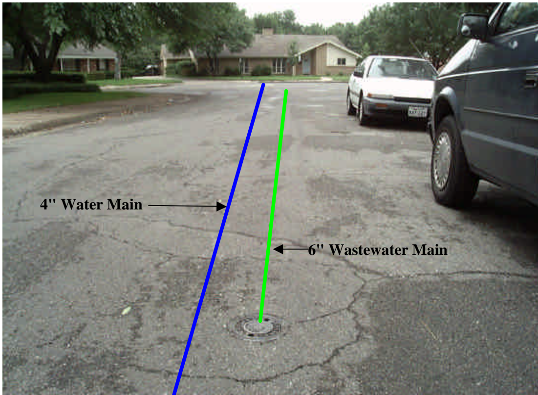
Figure 2 – Looking south at sanitary sewer cleanout on Ponder Place.
